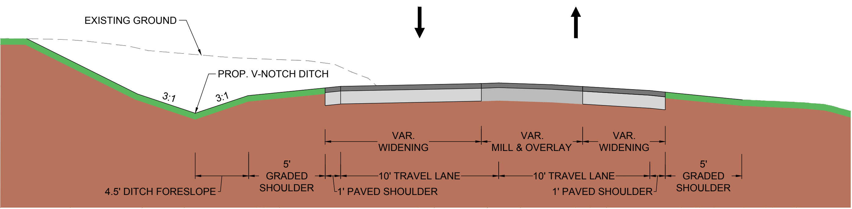
CARSON ROAD SECTION A-A WIDENING TO BOTH SIDES - BRIDGE APPROACH
