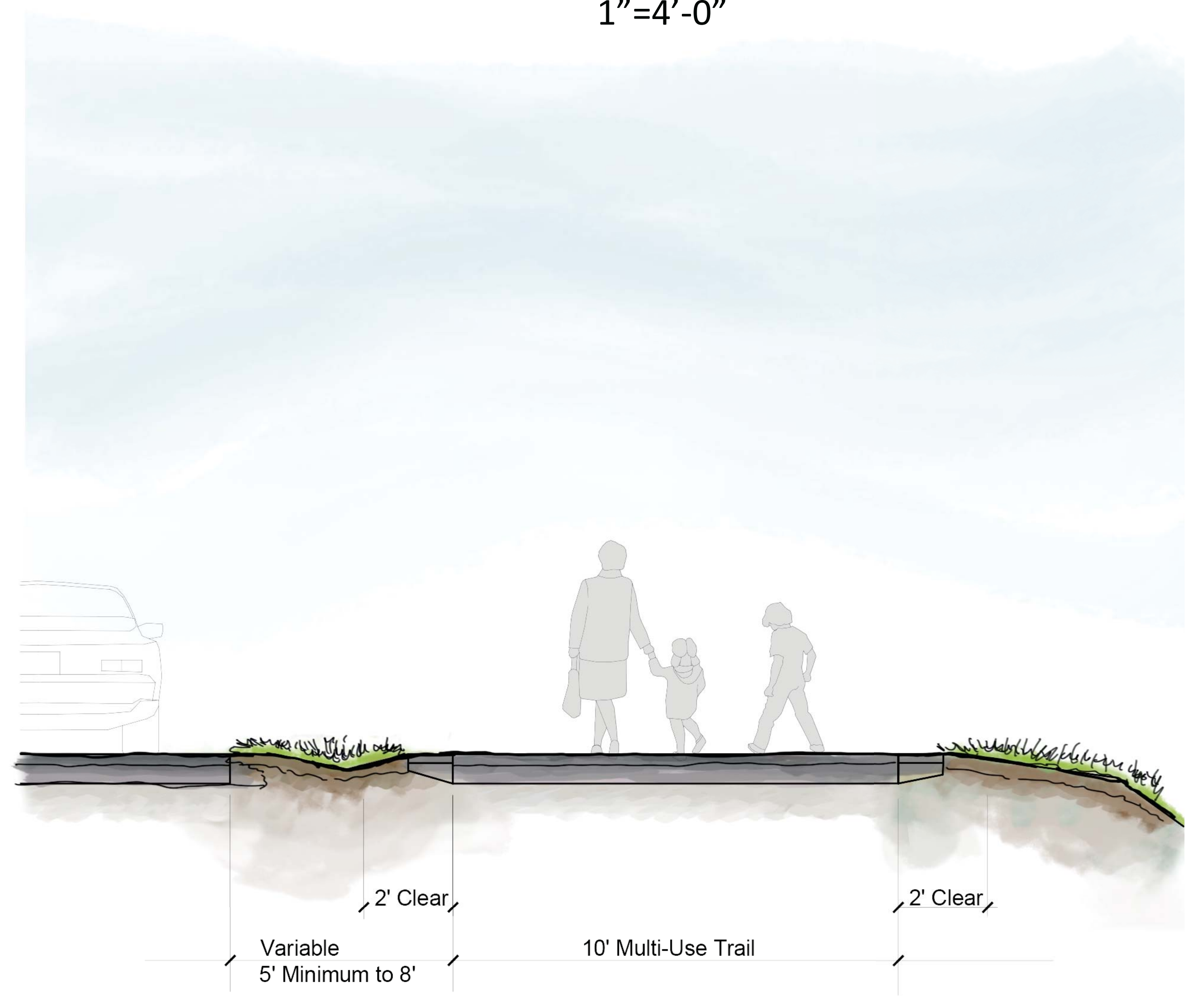
Multi-Use Trail Along Neighborhood Road 1"=2'-0"
