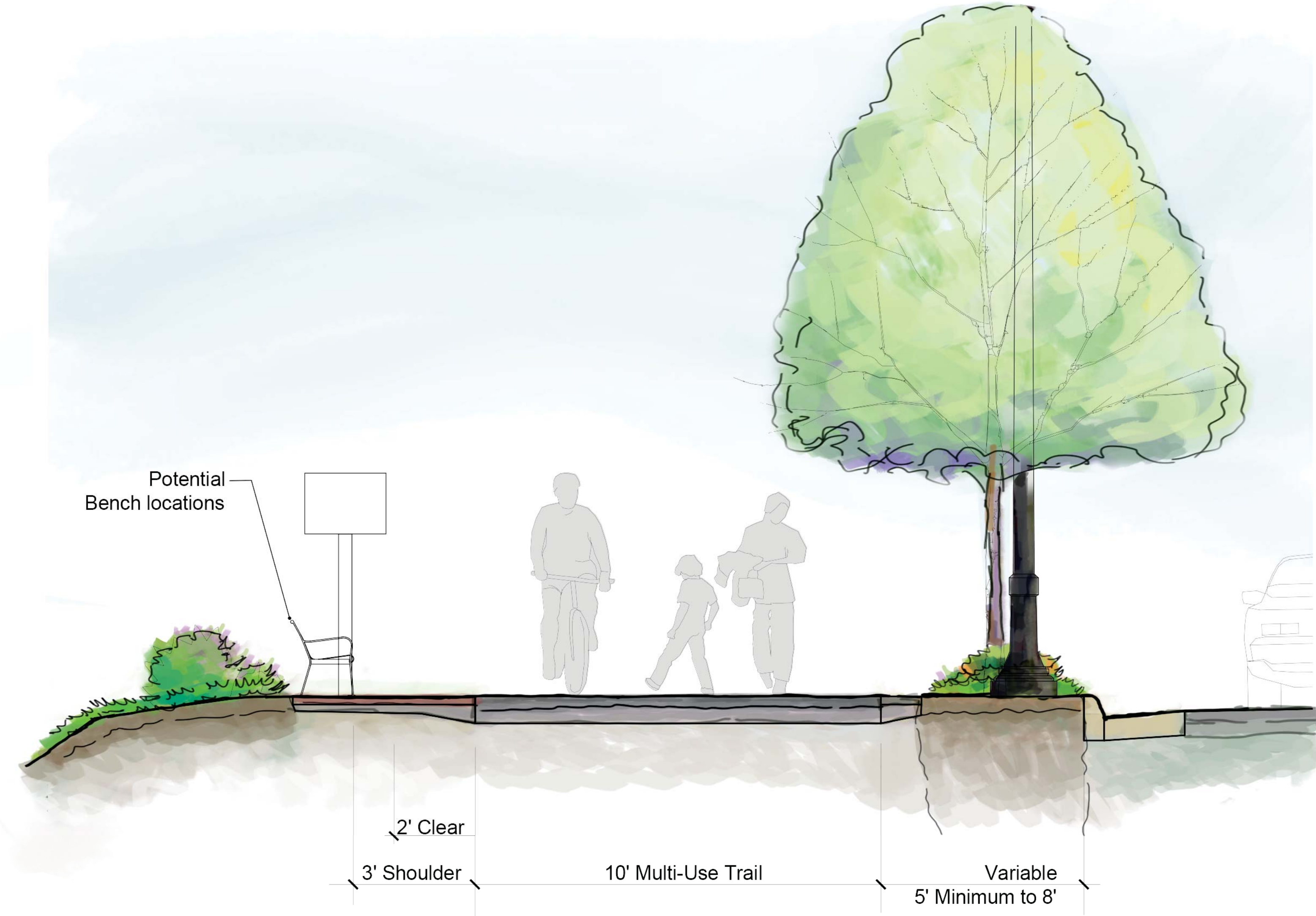
Multi-Use Trail Along Plantation Road 1"=2'-0"
