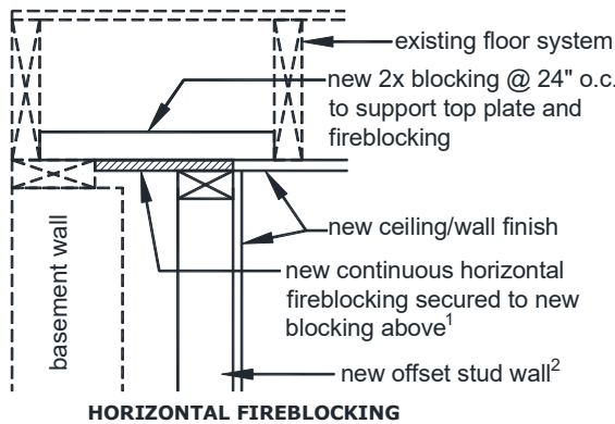
FIGURE 4: FIREBLOCKING WITH STUD WALL AGAINST BASEMENT WALL
